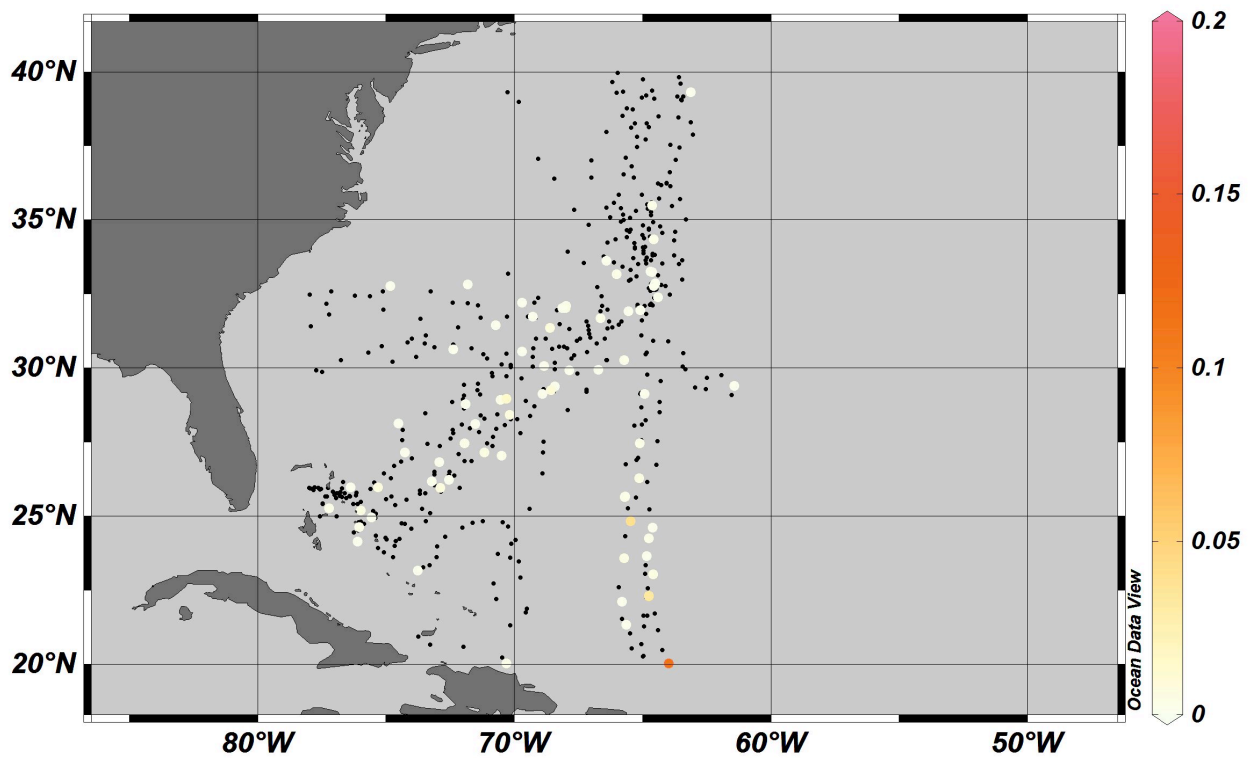
FIGURE 3. Distribution of eel larvae during fall (top panel) and spring (bottom panel) cruises (1977 – 2010). Color bar indicates density ( \text{g}/\text{m}^2 ). Black points indicate tows with an eel larvae density of 0 \text{ g}/\text{m}^2 .
